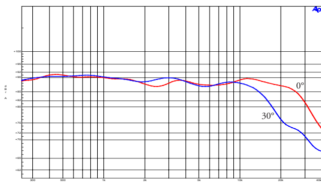
Frequency response: Also -30° out of axe vertical, very linear, excellent listening angle with APC. MK 3- System.
