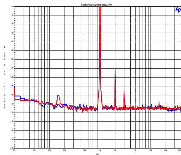
THD+ N 0 dB Signal, K_2 - 70 , K_3 - 95\text{dB}
